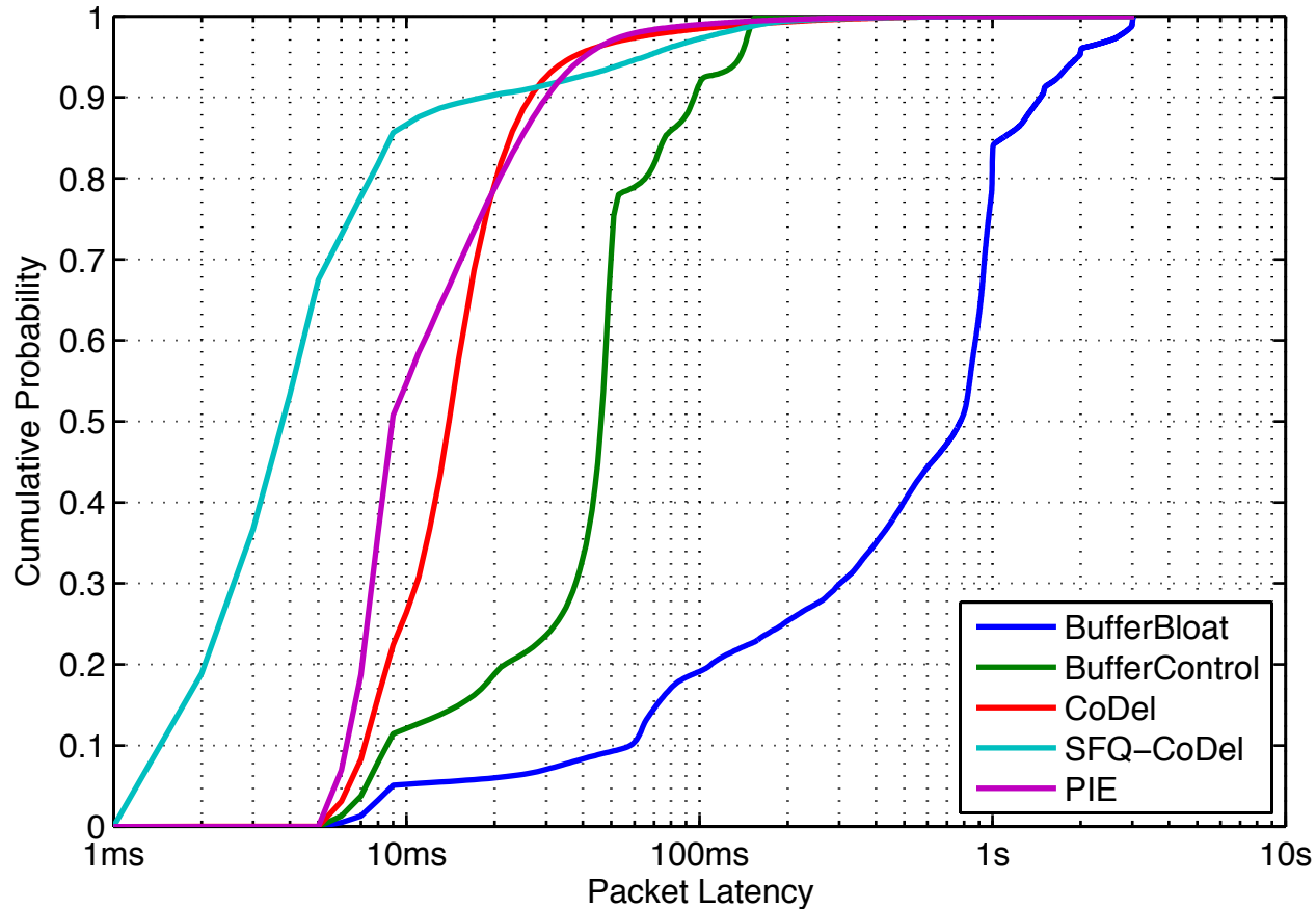
CDF of Gaming Traffic Packet Latency
